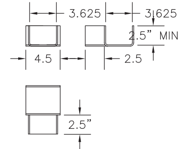
D T-BRACKET OPTION 1.0 SCALE: 1":1'
