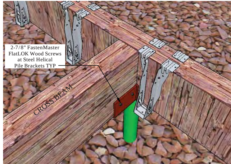
2 DETAIL AT CROSS BEAM CONNECTION Scale: NOT TO SCALE
