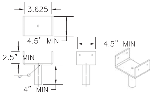
A STANDARD TMP BRACKET 1.0 SCALE: 1":1'
