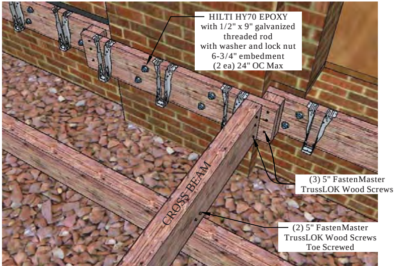
3 DETAIL AT LEDGER AROUND CHIMNEY Scale: NOT TO SCALE
