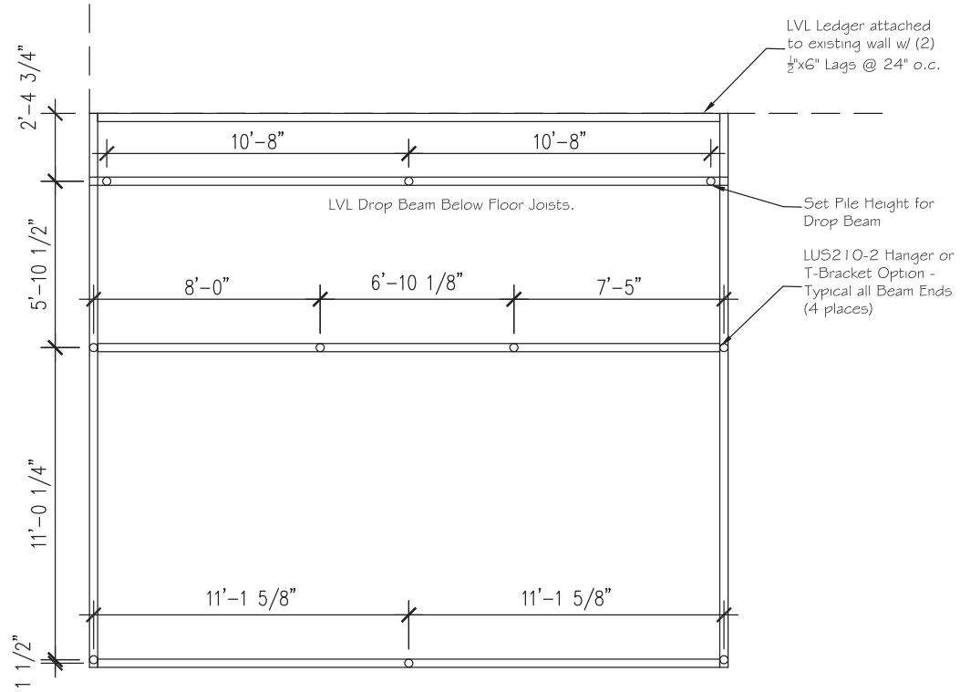
1 FOUNDATION PLAN 1.0 SCALE: 1/4":1'
