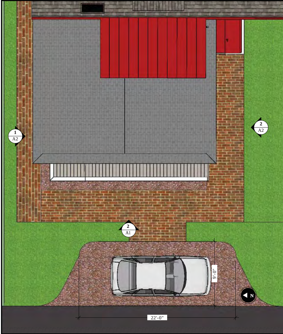
1 PLAN VIEW OF ROOFS Scale: 3/16" = 1'-0"
