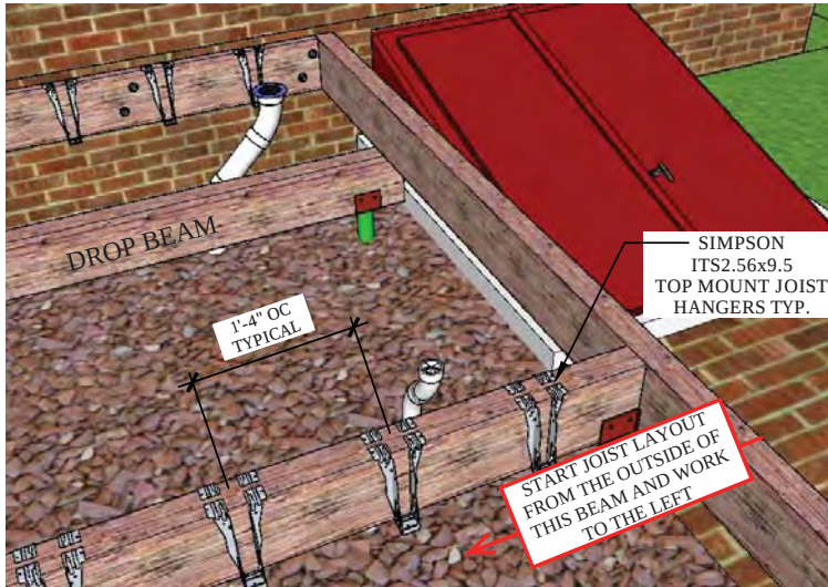
1 DETAIL AT JOIST HANGERS Scale: NOT TO SCALE
