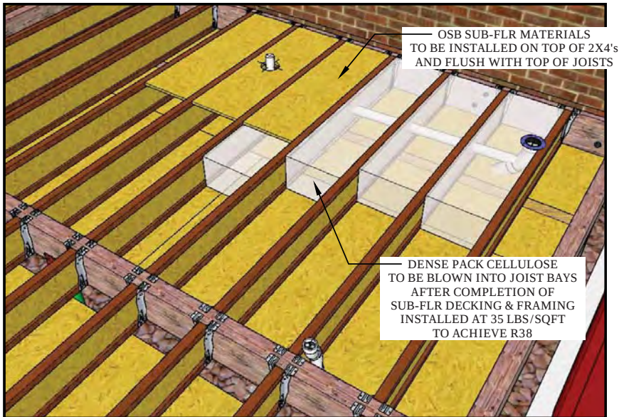
2 DECK ASSY INSULATION Scale: NTS
