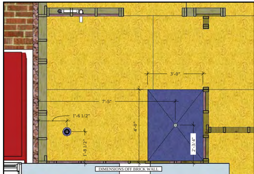
4 PVC PIPING & SHWR PAN LAYOUT Scale: NTS
