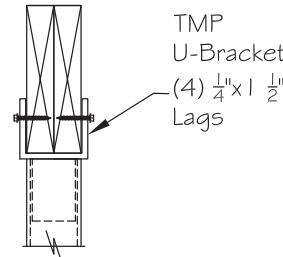
C INTERIOR BEAM SUPPORT 1.0 SCALE: 1":1'
