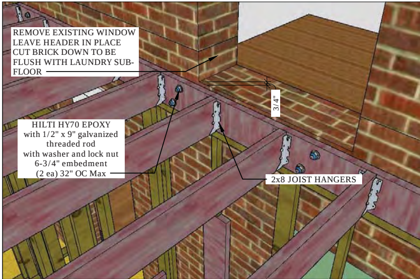
1 LAUNDRY FLOOR & DOOR OPENING Scale: NTS
