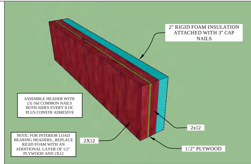
2 TYPICAL EXTERIOR WALL HEADER Scale: NTS
