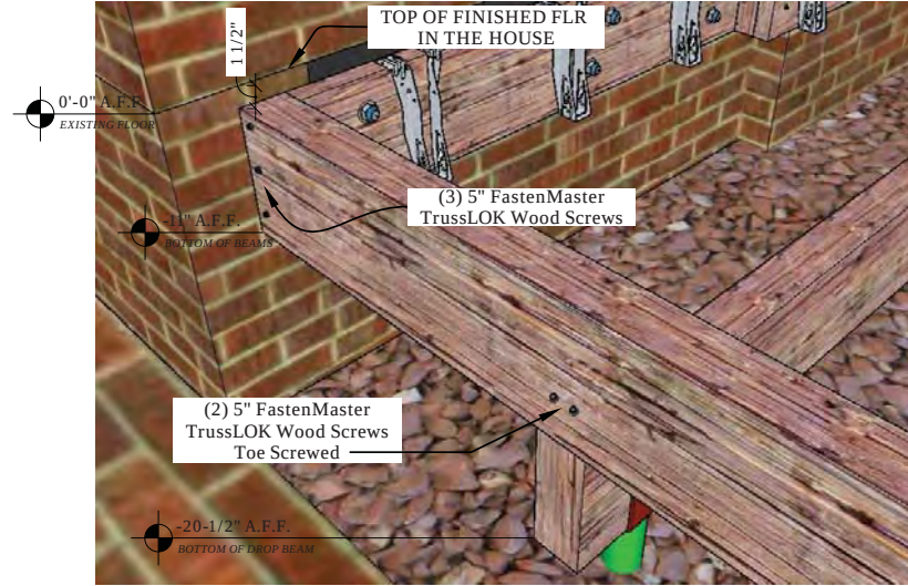
4 DETAIL AT BEAM END CONNECTIONS Scale: NOT TO SCALE
