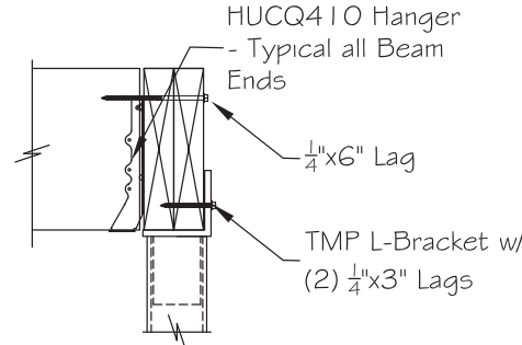
B EXTERIOR BEAM SUPPORT 1.0 SCALE: 1":1'
