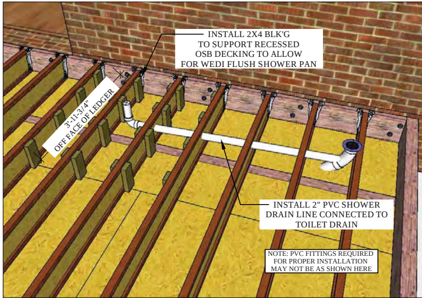
1 SHOWER PAN BLOCKING Scale: NTS
