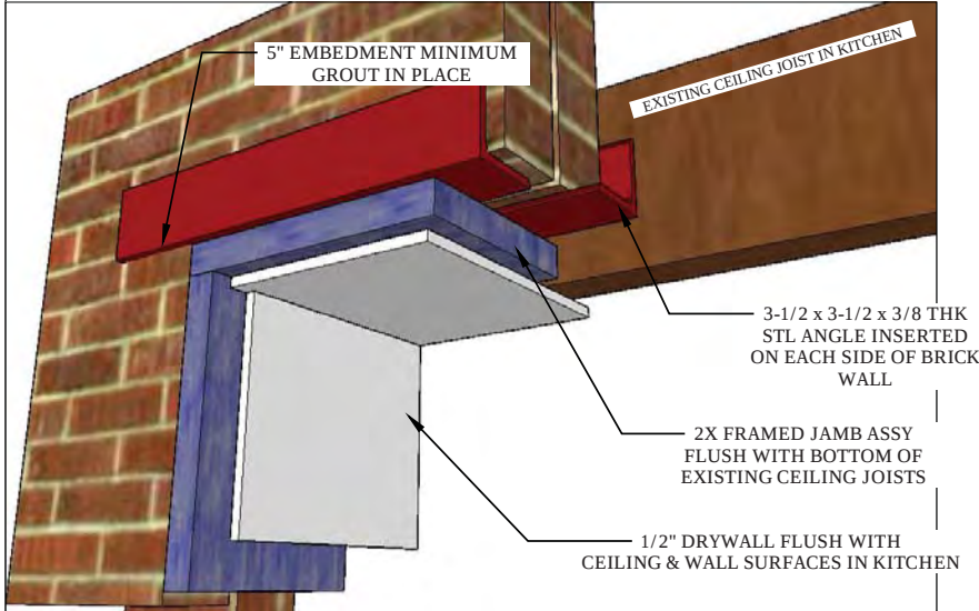
3 STEEL HEADER @ OPENING TO KITCHEN Scale: NTS
